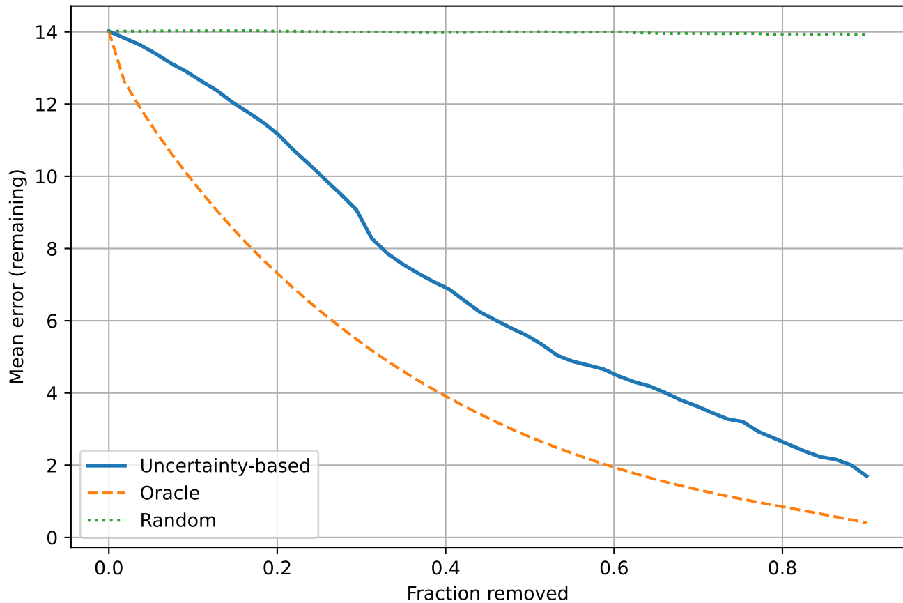
BPIC201D: Sparsification Curve
